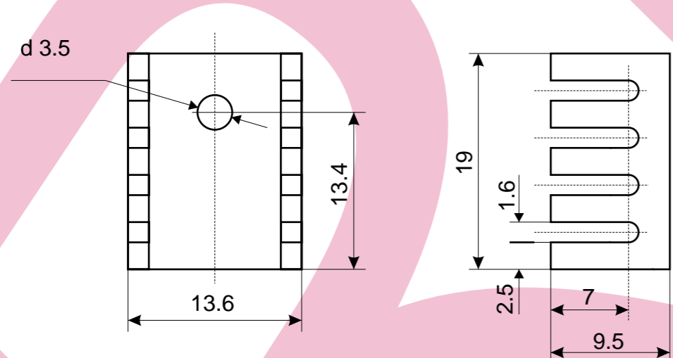
718 19x13.6x9.5 mm
