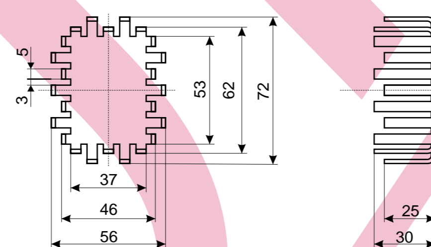
202 56x72x30 mm
