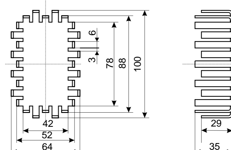
203 64x100x35 mm
