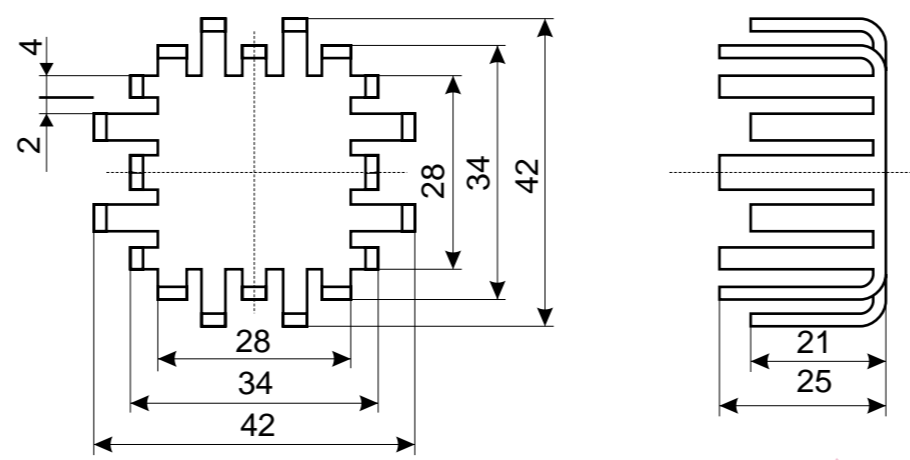
102 42x42x25 mm
