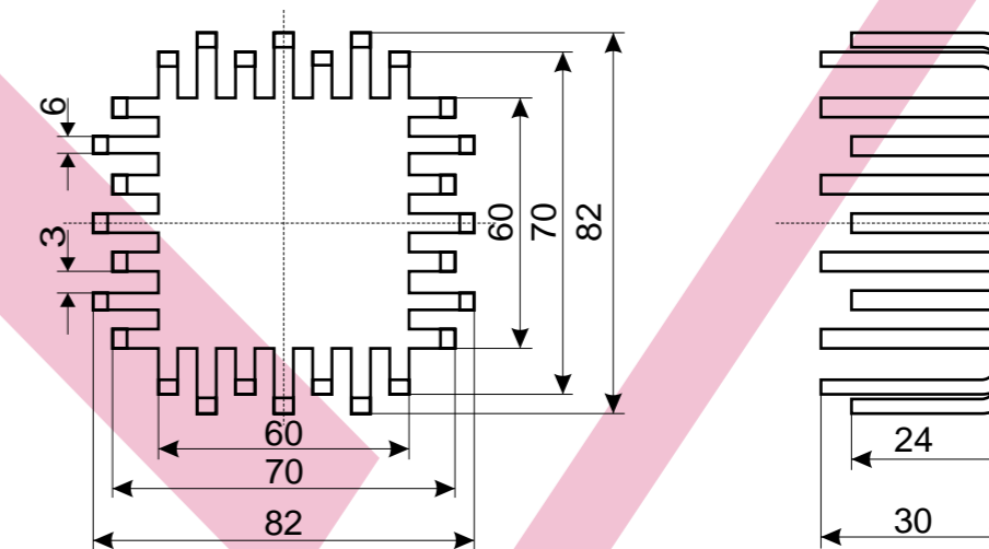
106 82x82x30 mm
