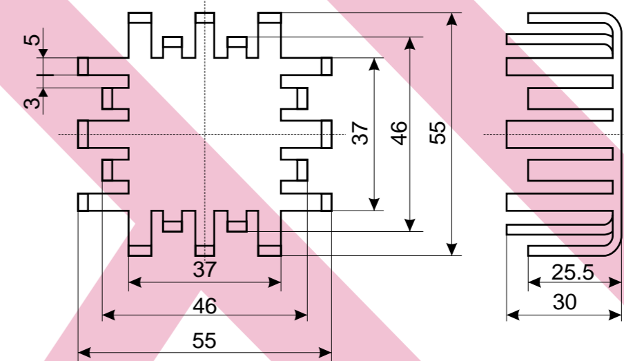
103 55x55x30 mm
