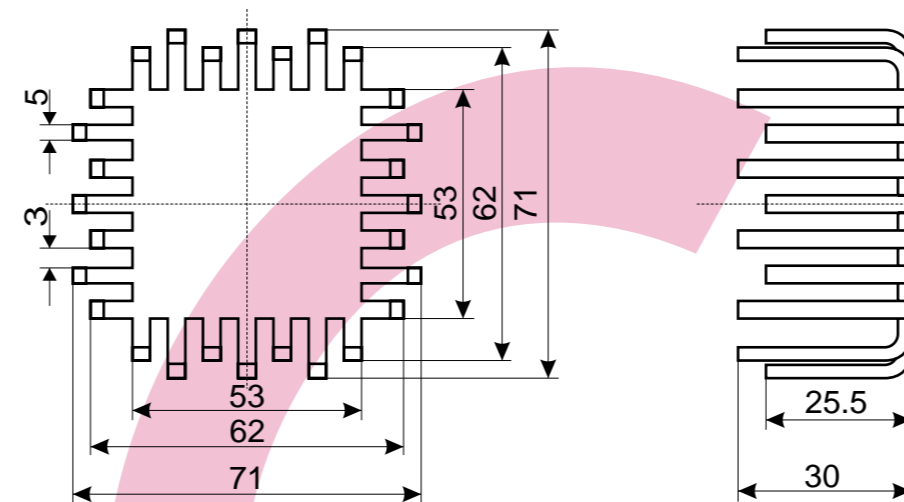
105 71x71x30 mm
